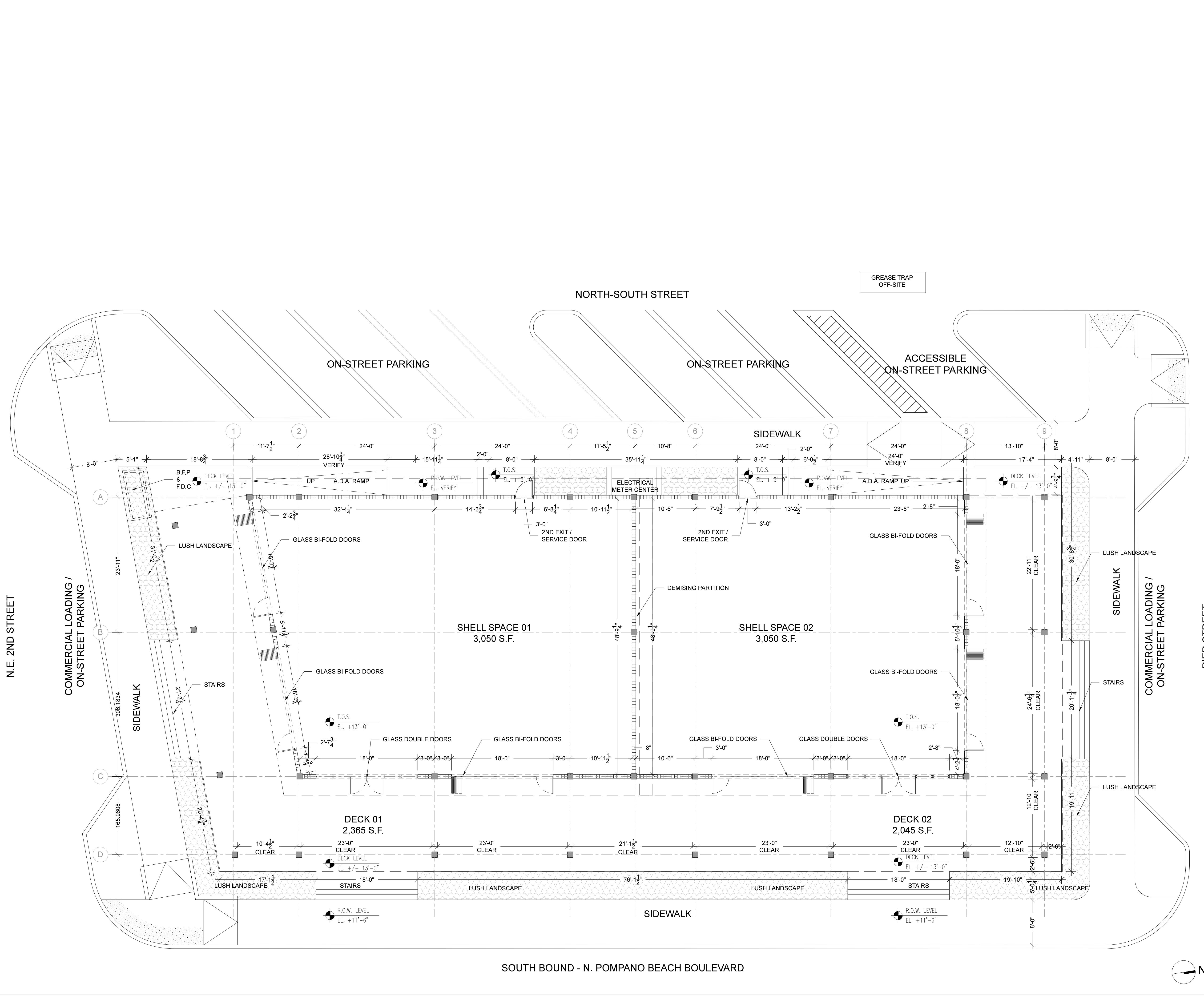
01 FIRST FLOOR PLAN SCALE: 1/8"=1'-0"
